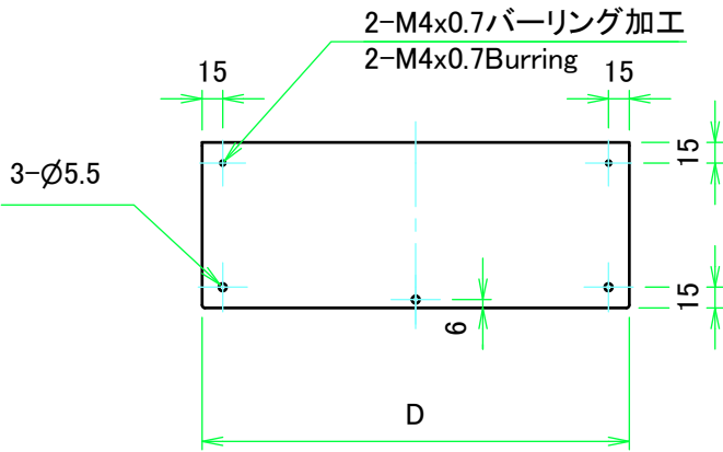
C view
