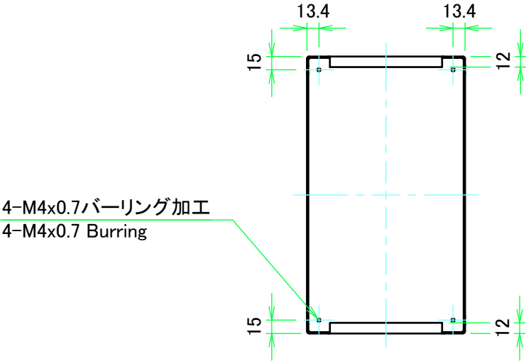
E view
