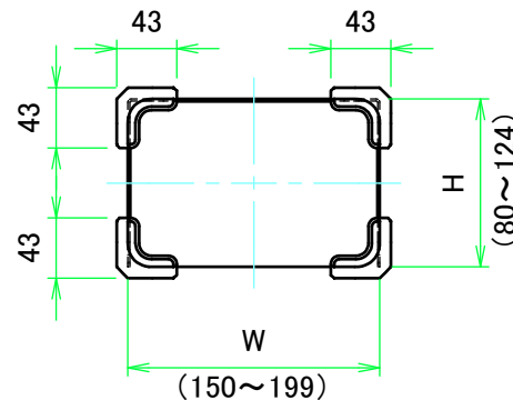
A view
