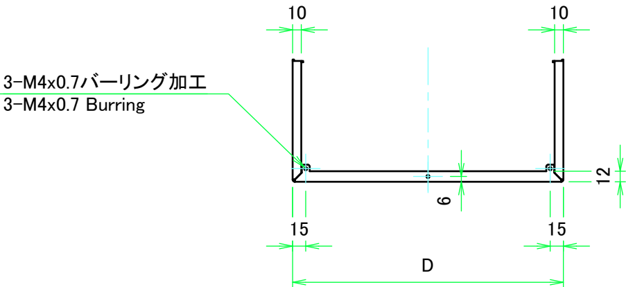
C view
