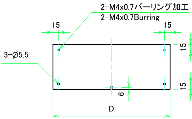
C view
